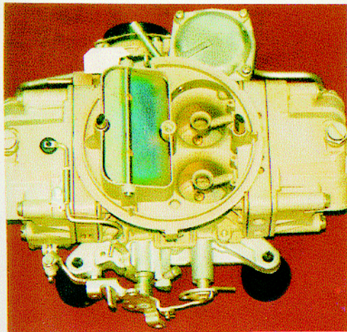
HOLLEY 4150
