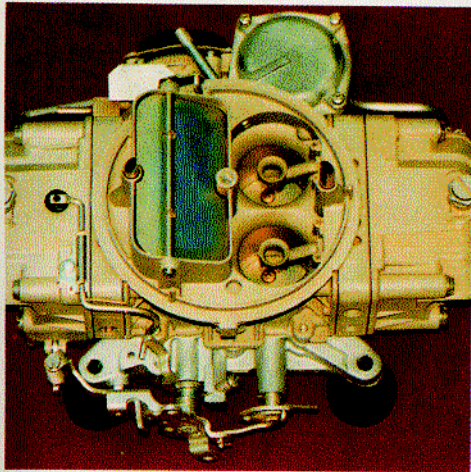
HOLLEY 4150
