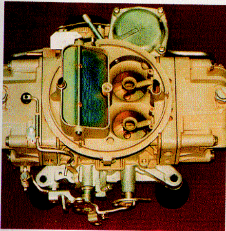
HOLLEY 4150
