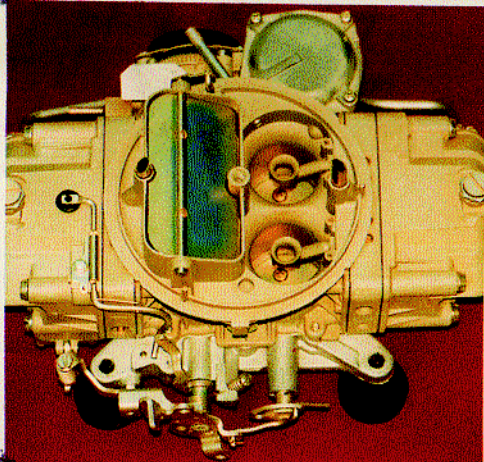
HOLLEY 4150
