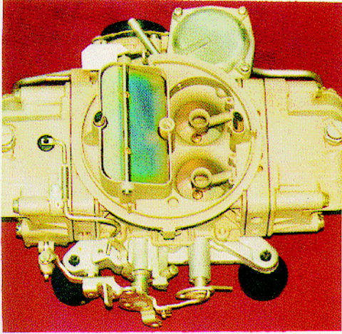
HOLLEY 4150
