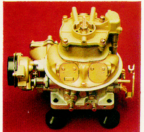
HOLLEY 4000 "TEAPOT"
