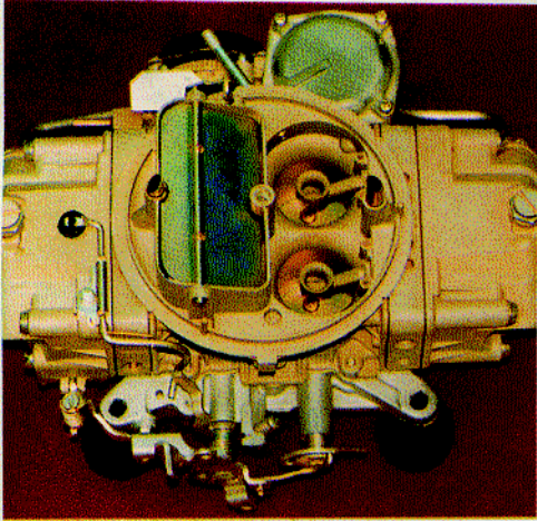
HOLLEY 4150
