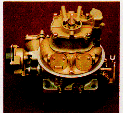
HOLLEY 4000 "TEAPOT"
