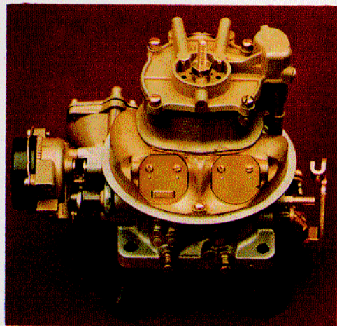
HOLLEY 4000 "TEAPOT"
