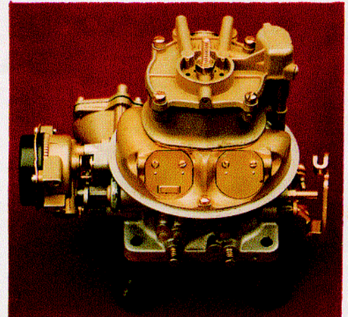
HOLLEY 4000 "TEAPOT"
