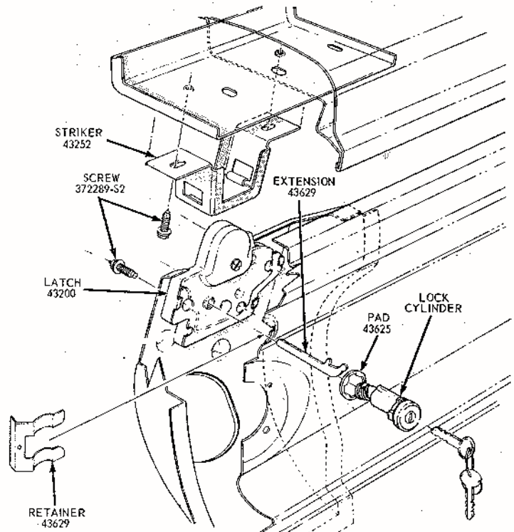
1969 MUSTANG LUGGAGE COMPARTMENT LATCH MECHANISM.....
