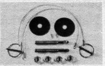
Hood Latch Kit —65/66 ..... 14.95
